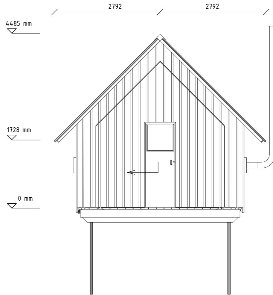
Front elevation
