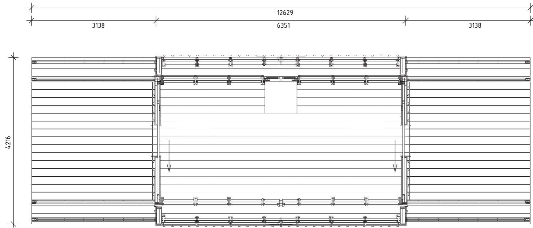
Floor plan-Ground floor
