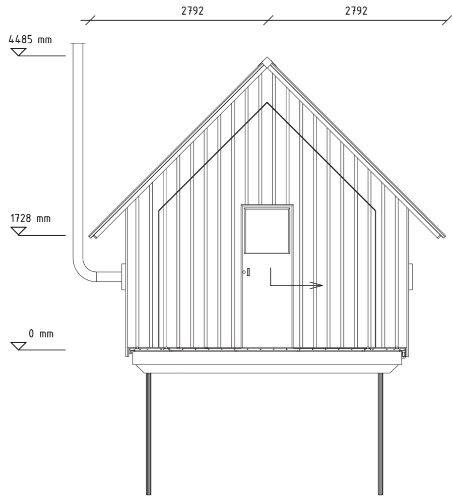
Back elevation
