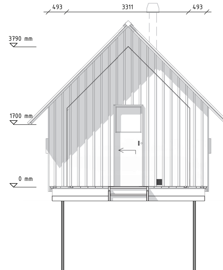
Front elevation
