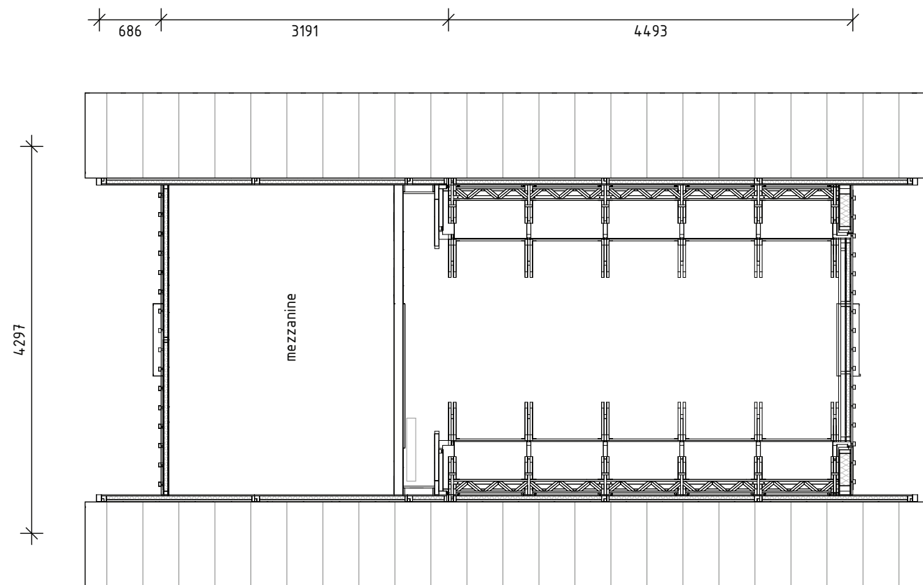
Floor plan-Mezzanine
