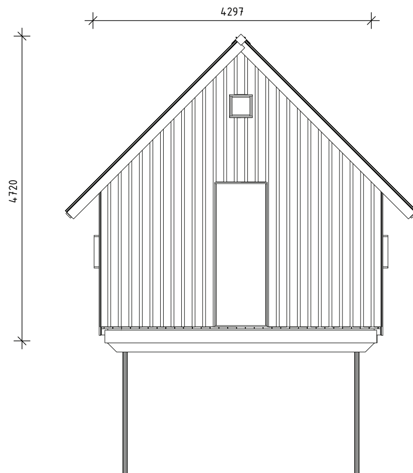
Back elevation
