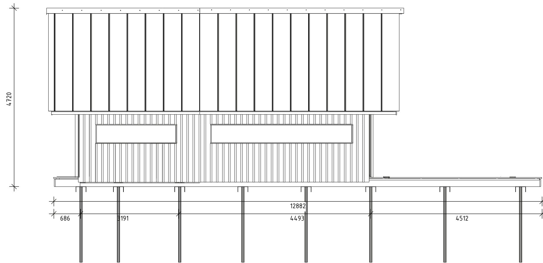
Side elevation
