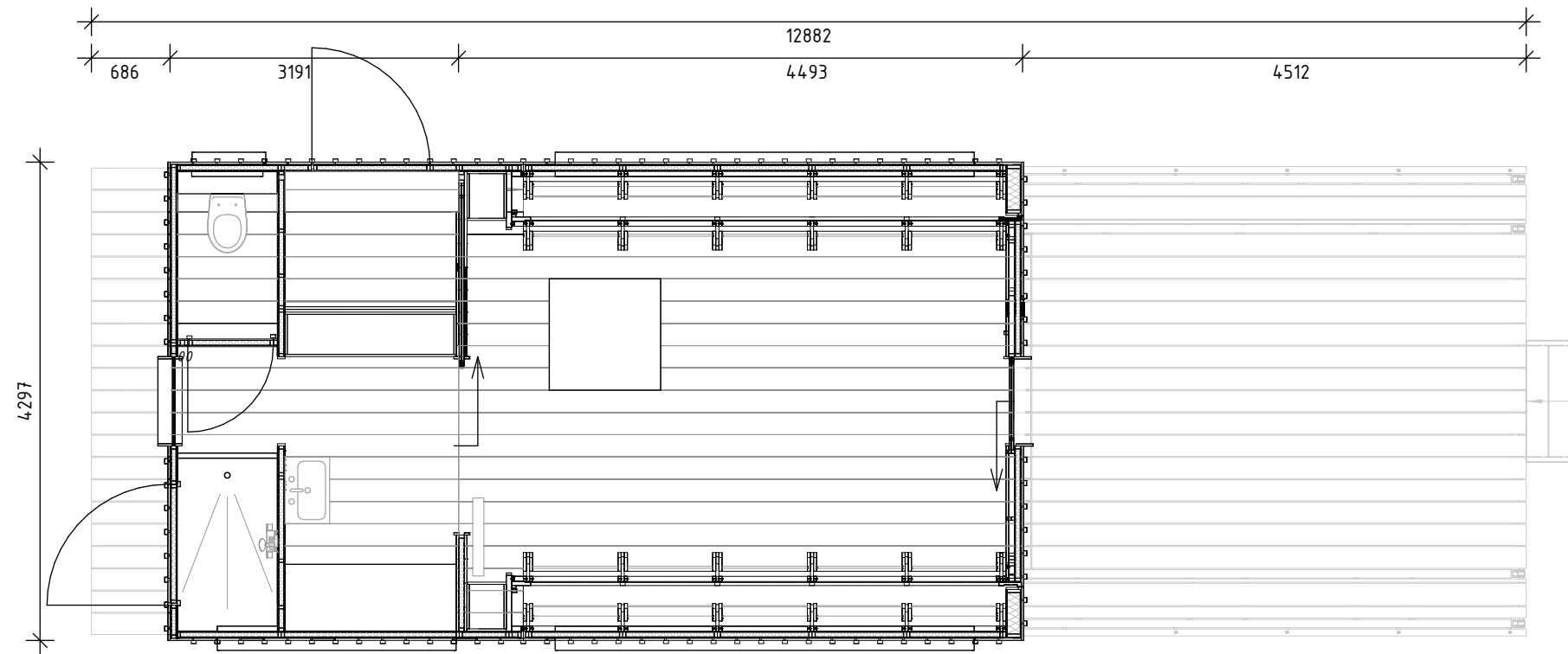
Floor plan-Ground floor
