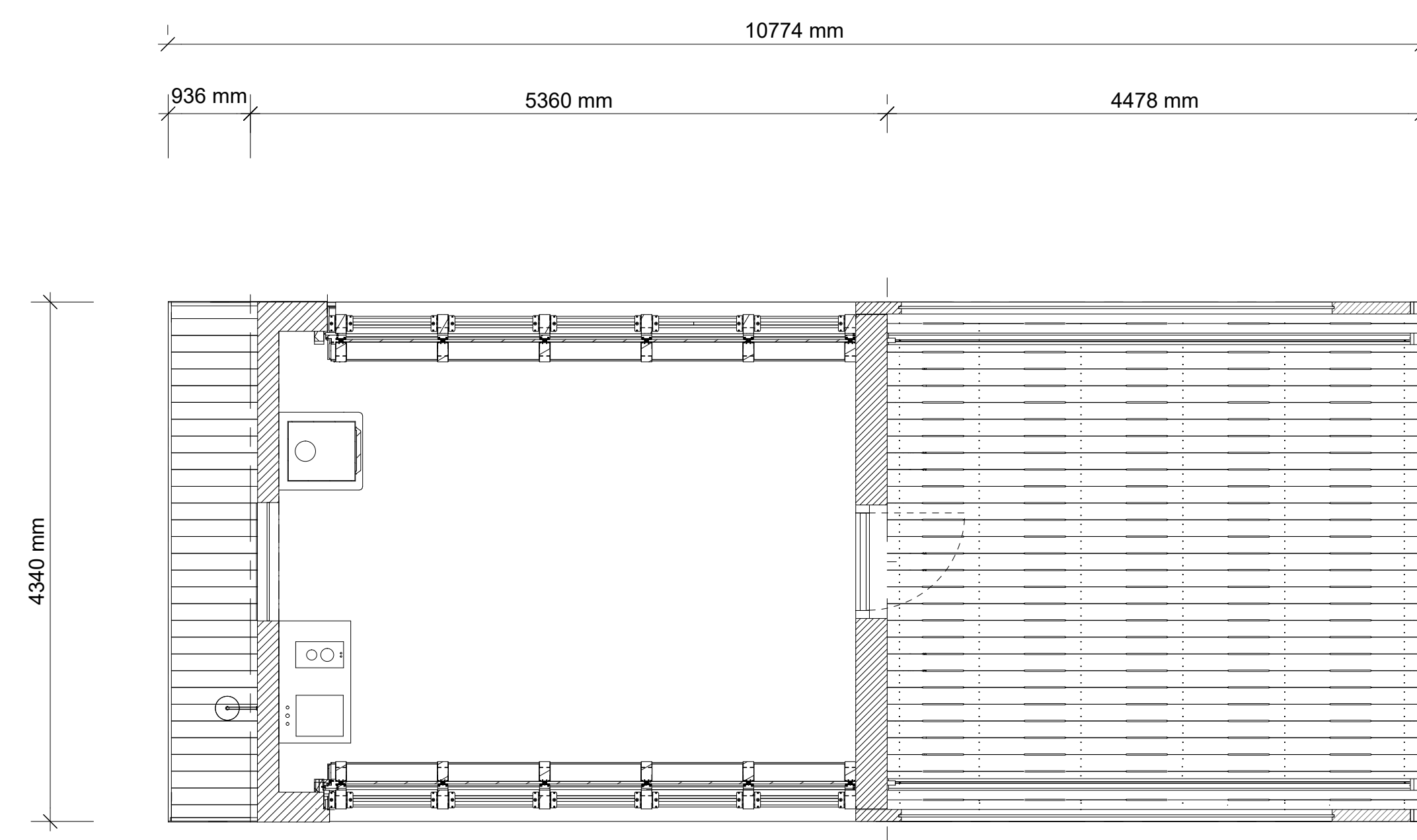
Floor plan – Ground floor
