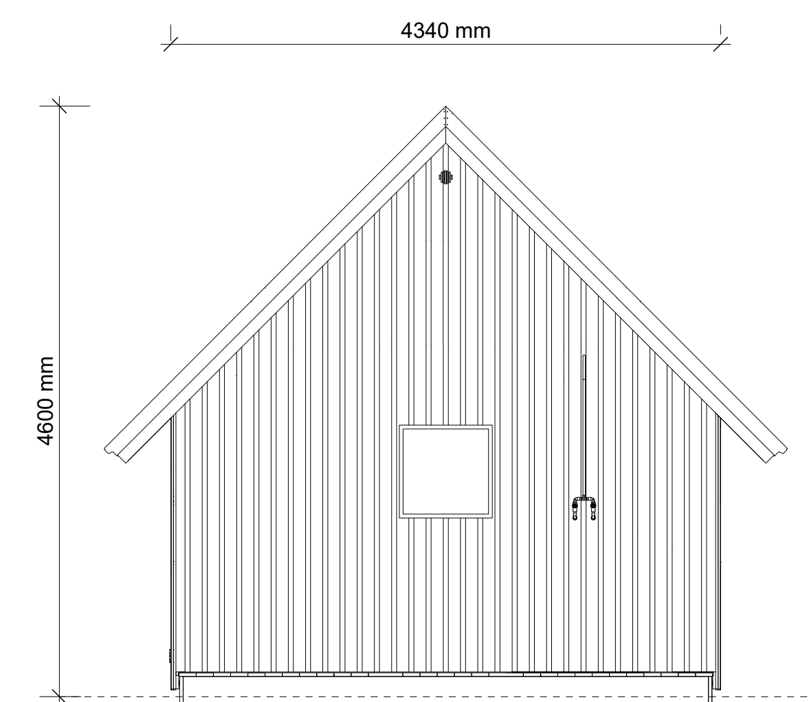
Back elevation
