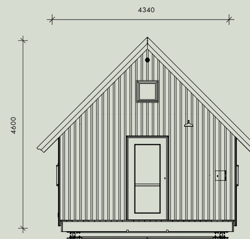
Back elevation
