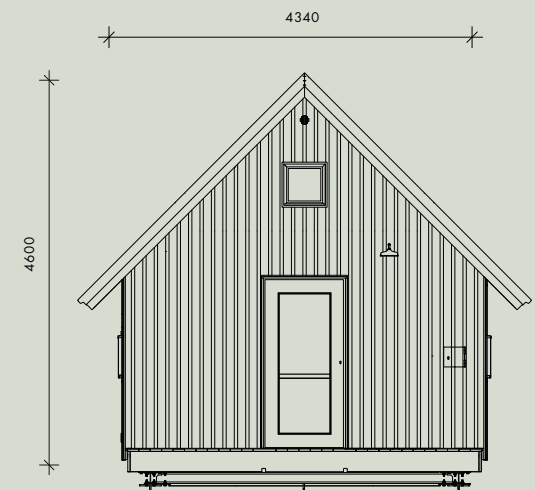
Back elevation
