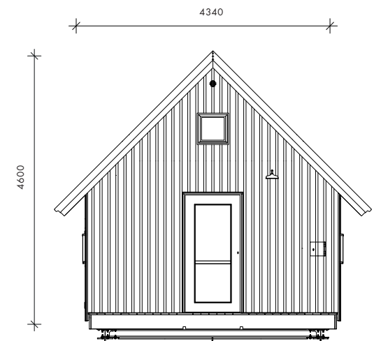
Back elevation
